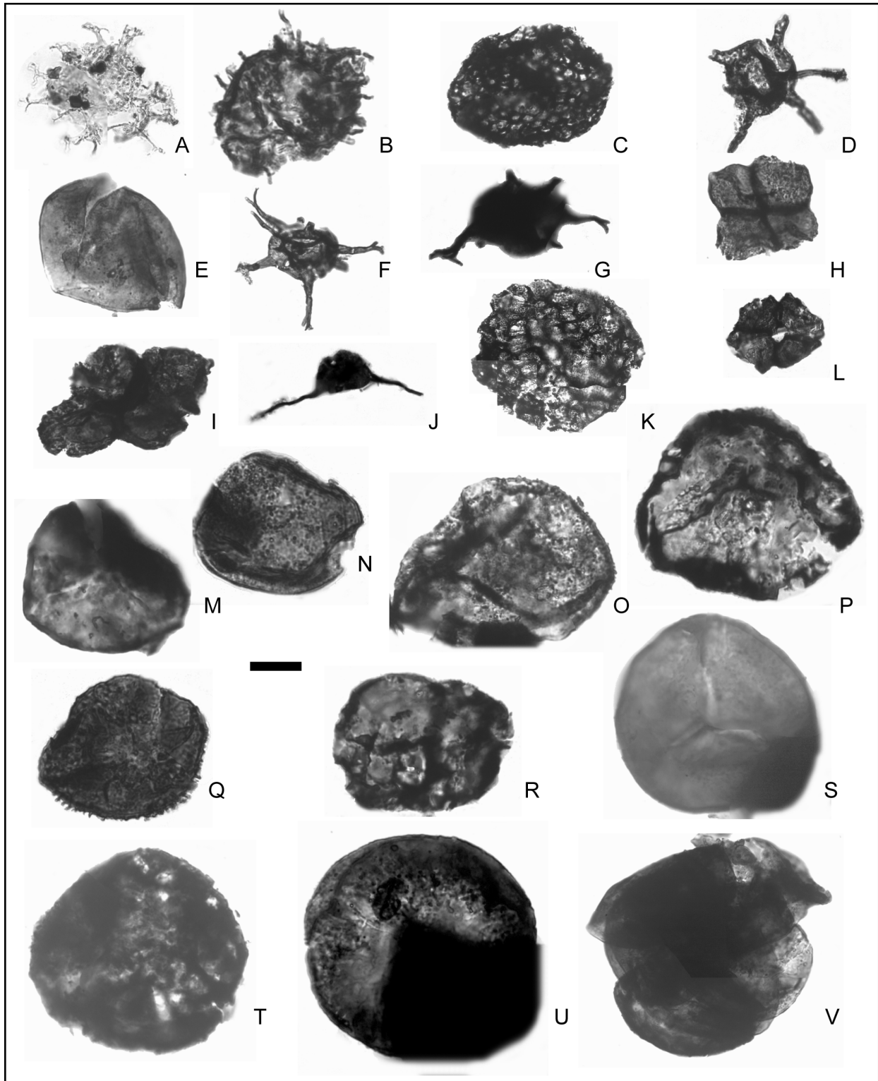
Figure 4. A, Ammonidium garrasinoi (BAFC-PI 2086(1), EF: Y43/1); B, Baltisphaeridium? sp. (BAFC-PI 2091(1), EF: F48); C, Dictyotidium variatum (BAFC-PI 2091(1), EF: V52/3); D, Exochoderma arca (BAFC-PI 2089(1), EF: T49/3); E, Leiosphaeridia sp. (BAFC-PI 2086(1), EF: C26); F, Multiplicisphaeridium ramusculosum (BAFC-PI 2091(1), EF: B48/2); G, ? Multiplicisphaeridium sp. (BAFC-PI 2087(1), EF: C32/2); H, Quadrisporites granulatus (BAFC-PI 2092(1), EF: X46); I, Quadrisporites variabilis (BAFC-PI 2092(1), EF: V38/1); J, Veryhachium sp. (BAFC-PI 2087(1), EF: C41); K, ?Algal coenobium A (BAFC-PI 2092(1), EF: W34/1); L, Algal coenobium B (BAFC-PI 2092(1), EF: Z38/3); M, Ambitisporites avitus/dilutus morphon BAFC-PI 2086(1), EF: U51/1); N, Apiculatasporites sp. (BAFC-PI 2086(1), EF: C25/1); O, Apiculiretusispora sp. (BAFC-PI 2086(1), EF: E25/3); P, Cymbosporites sp. (BAFC-PI 2090(1), EF: O31/2); Q, Dibolisporites farraginis (BAFC-PI 2086(1), EF: B27/2); R, Dyadospora sp. (BAFC-PI 2090(1), EF: S26); S, Retusotriletes sp. (BAFC-PI 2086(1), EF: G55/3); T, Retusotriletes sp. cf. R. maculatus (BAFC-PI 2090(1), EF: Q23/3); U, ? Scylaspora costulosa (BAFC-PI 2086(1), EF: E40); V, Tetrad (BAFC-PI 2086(1), EF: Z27/2). Scale bars: A, C-J, V = 20 \mu m.; B = 10 \mu m.; K, L = 35 \mu m.; M-U = 15 \mu m.
