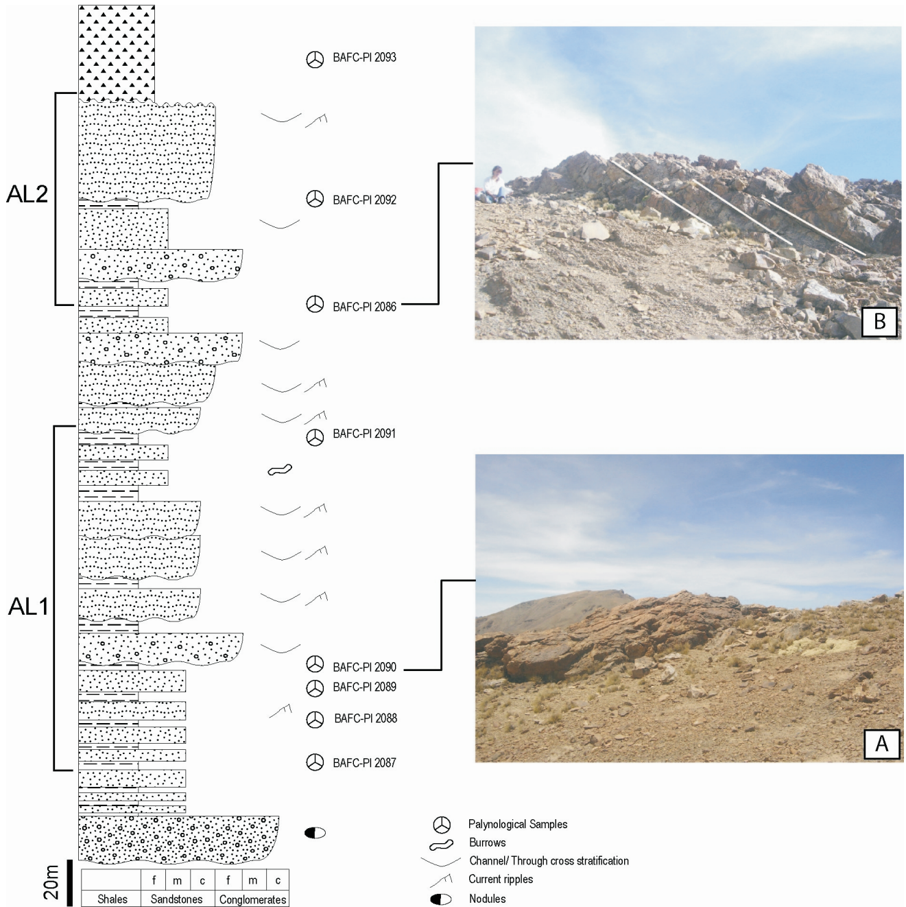
Figure 2. Stratigraphic section from the Abra Limite locality with the position of the studied samples, quoted with the BAFC-PI acronym. A , channel over the fine sandstones and shale from where the sample BAFC-PI 2090 was collected; B , channel erosive contact over fine sandstones and shales and lateral accretion surfaces. Abbreviations: AL1, palynoassemblage 1; AL2, palynoassemblage 2.
