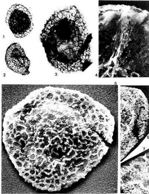
Fig. 2. Original reproduction of Plate IV from STEEMANS et al. (1996). 1, 5. Retispora lepidophyta (KEDO) PLAYFORD 1976; 1. Evioux Formation, Langlier Quarry, Dinant Basin, Belgium, x 500; 5. SEM photo showing muri and additional ornament, well visible at the equator, x 2.500. 2, 6, 7. Retizonomonoletes hunanensis FANG et al., 1993; 2. Oujiaichong Formation, Malanbian, Hunan, x 500; 6-7. SEM photo showing density of ornamentation, x 2.500. 3, 4. Retispora macroreticulata (KEDO) BYVSHEVA 1985; 3. Evioux Formation, Evioux railway section, Dinant Basin, Belgium, x 500; 4. SEM photo showing muri and additional apiculate ornament, x 2.500.
